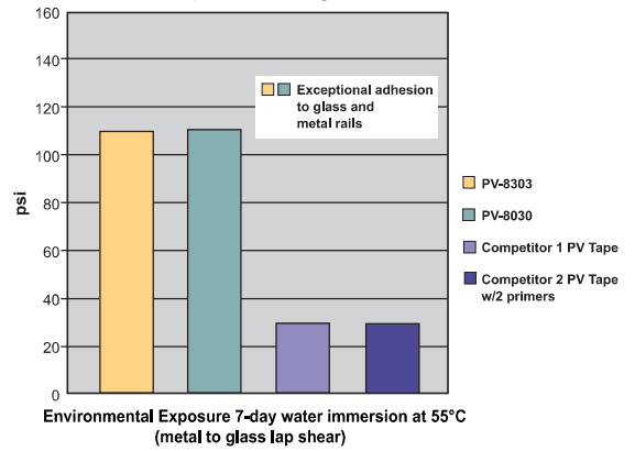
Dow Corning Rail Bonding Solutions vs. PV Tapes Lap Shear Strength
