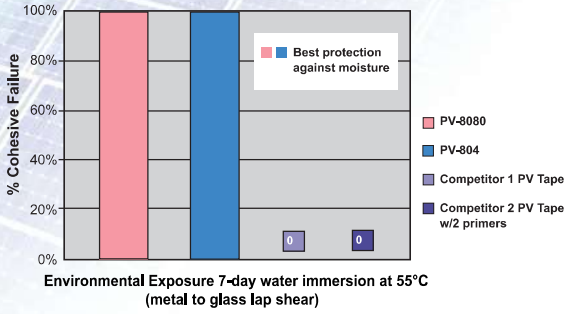
Dow Corning Frame Sealing Solutions vs. PV Tapes Cohesive Failure
