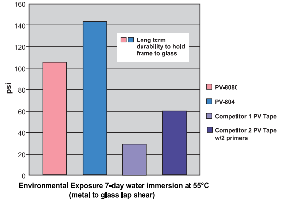
Dow Corning Frame Sealing Solutions vs. PV Tapes Lap Shear Strength
