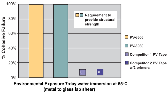
Dow Corning Rail Bonding Solutions vs. PV Tapes Cohesive Failure
